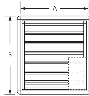
DETAIL #1 Single panel damper for ventilator size 36 & smaller.
