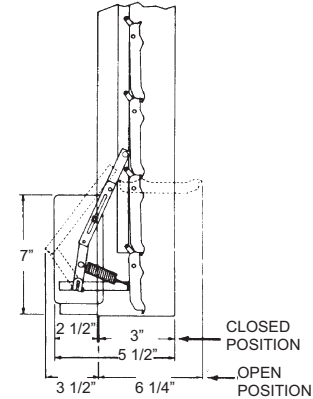
*Side view of shutter frame and installed motor pack
