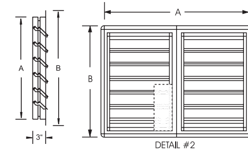
Two panel shutter for fan size 42 & larger
