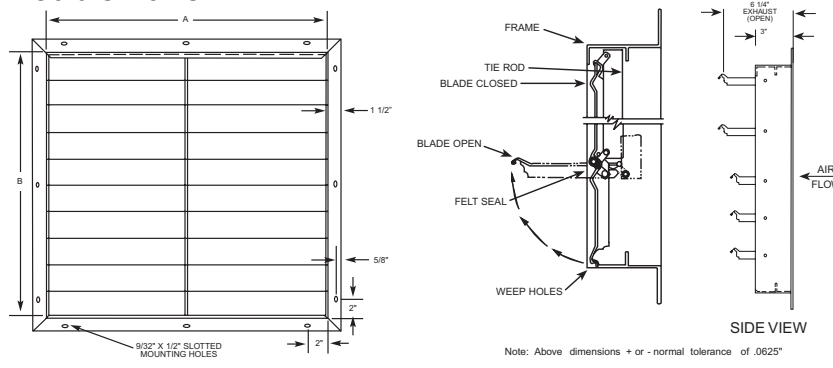
*Side view of shutter frame and installed motor pack
