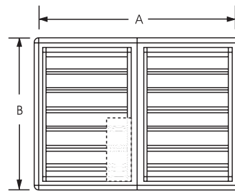
DETAIL #2 Two panel damper for ventilator size 42 & larger.
