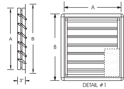
Single panel shutter for fan size 36 & smaller
