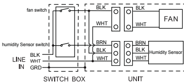
Fan with PCSC
