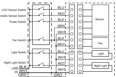
Fan with PCIAQS and PCLK / PCLEDK
