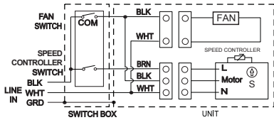
Fan With PCHS and PCLK / PCLEDK
