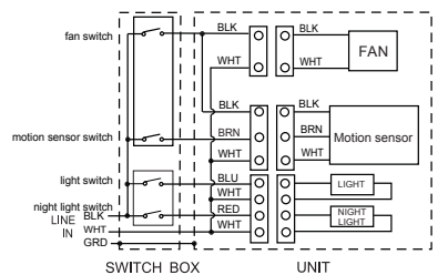
Fan with PCIAQS and PCLK / PCLEDK
