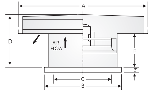
Model HRED-C Direct Drive (Hoods on 42" - 60" ship KD) (2) Specify assembled if required
