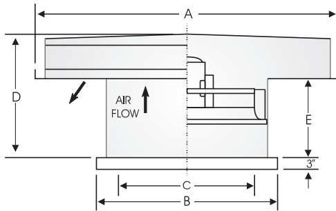
Model HREB-C Belt Drive (Hoods on 42" - 72" ship KD) (2) Specify assembled if required
